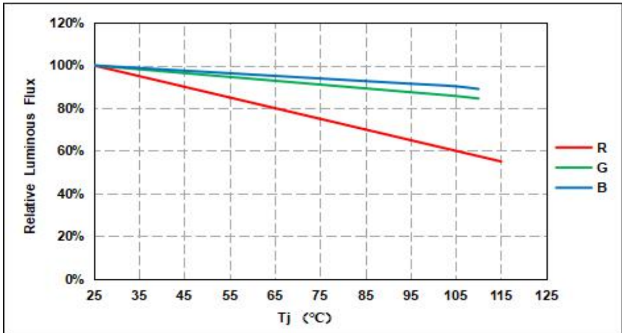
Relative Luminous Intensity VS Junction Temperature (IF=150mA, 25°C)
