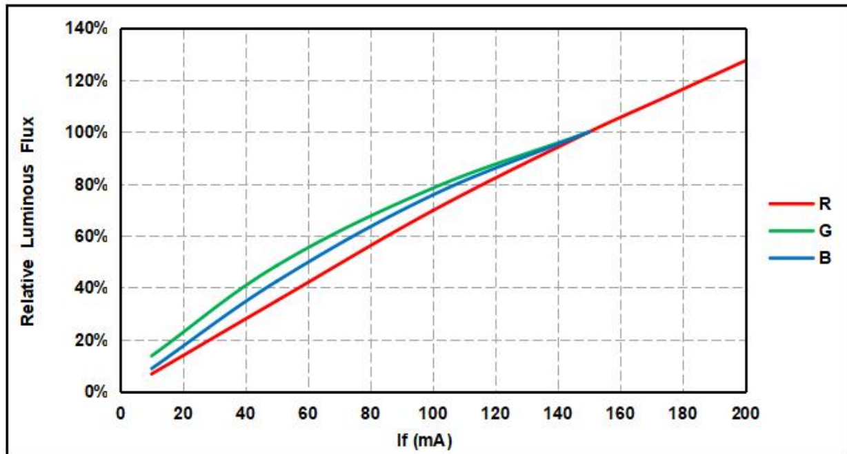
Relative Luminous Intensity VS Forward Current (IF=150mA, 25°C)
