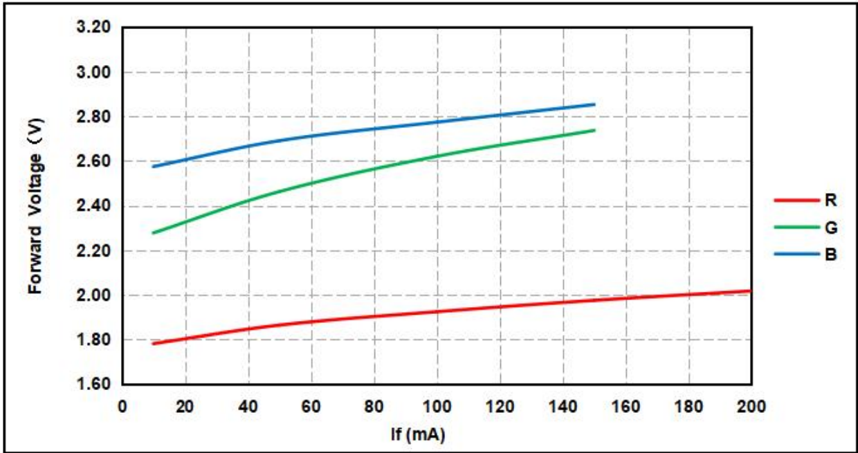
Forward Voltage VS Forward Current (IF=150mA, 25°C)
